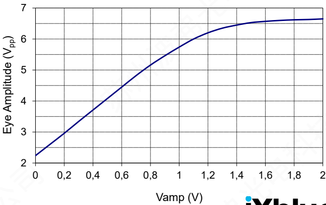
Typical Output Voltage Amplitude VS Gain Control Vamp Tuning Conditions: V_{bias} = 8\text{ V} , V_{xp} = 2\text{ V}
