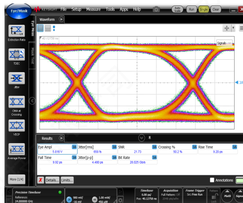
Output response Eye amplitude = 5.8\text{ V}_{pp}
